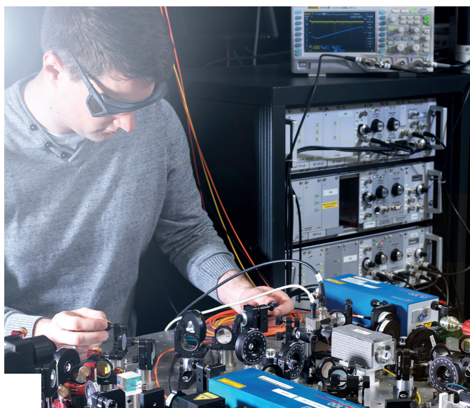
Measuring the nuclear properties of thorium-229, to be used as nuclear clock. [Credit PTB, Germany].
