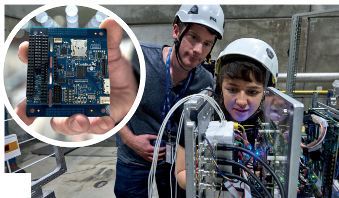
ESA's AI chip, Myriad 2, about to be tested for the effects of space radiation using the proton beam from CERN's SPS accelerator.
