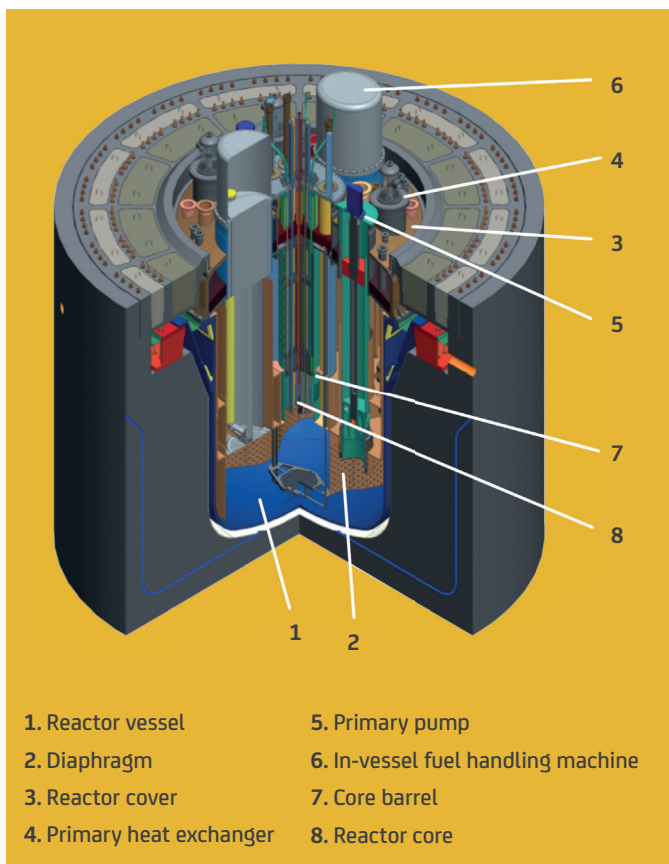
A graphic of the layout of the accelerator-driven system. [Credit SCK-CEN].
