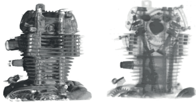
The neutron image of a working motorcycle engine. [Credit Paul Scherrer Institut].
