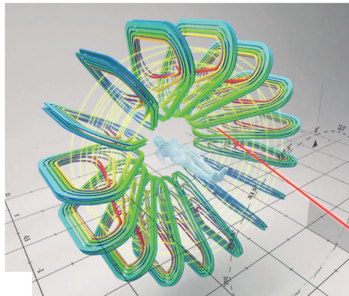
CERN is developing a new compact non-rotating gantry design for hadron therapy that can rotate the beam around the patient and reach tumours from different angles. It uses superconducting toroidal magnets.
