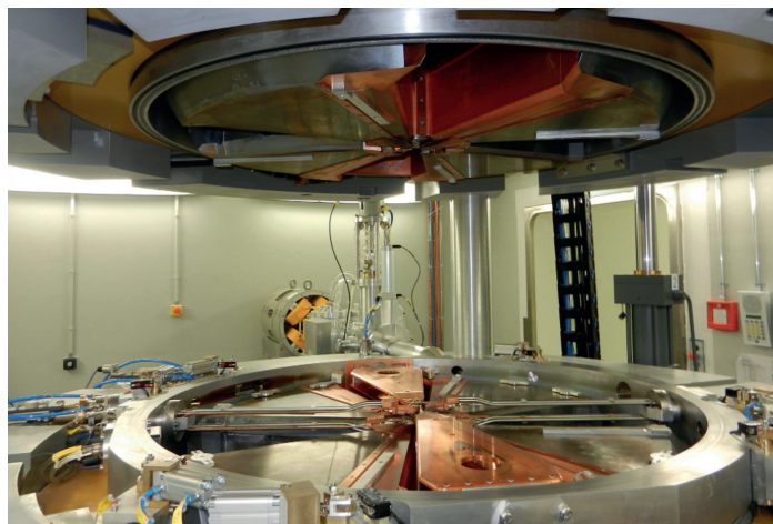
■ Inside the cyclotron used to make medical radioisotopes at the University of Bern Hospital in Switzerland.
