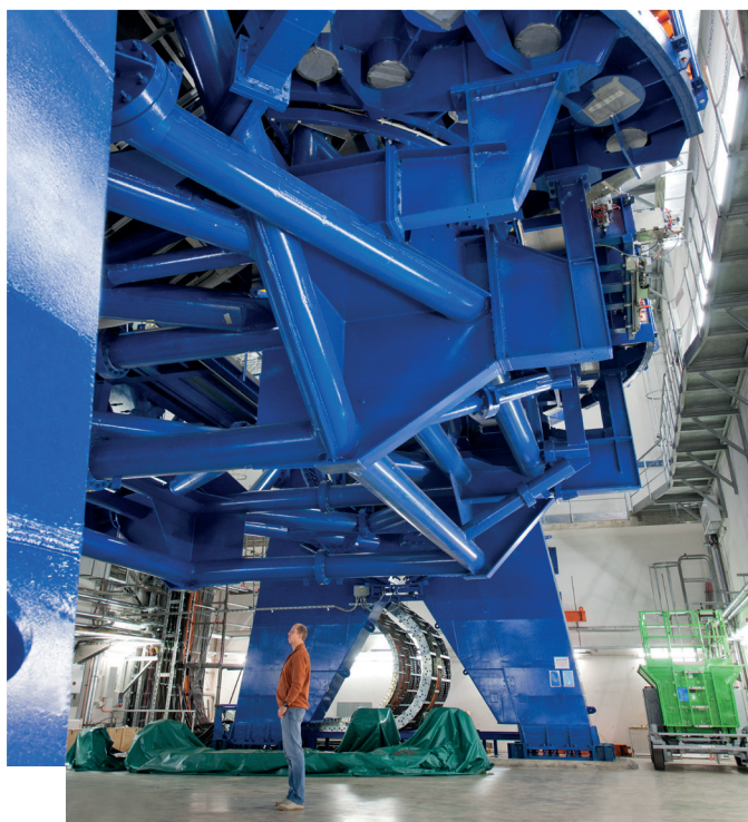
The massive gantry used to deliver ground-breaking carbon-ion therapy at the Heidelberg Ion Therapy Centre in Germany. More compact designs are now being developed. [Credit HIT].
