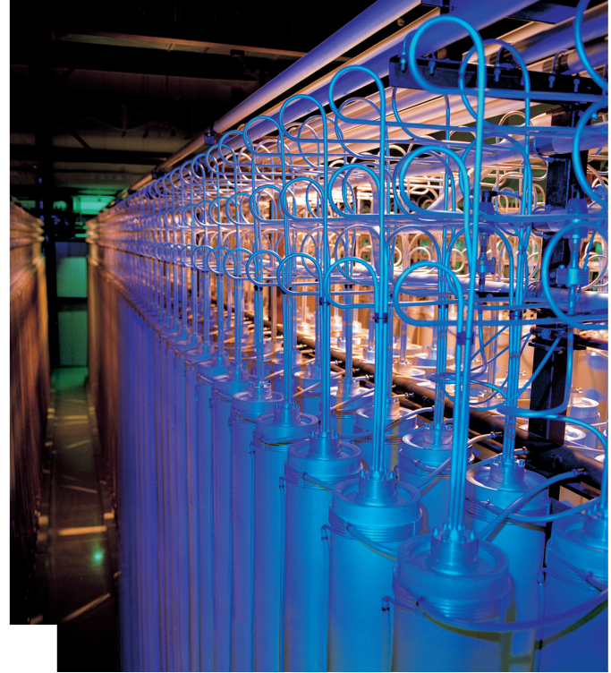
Centrifuges are used to separate uranium 235 from uranium-238. [Credit Urenco].
