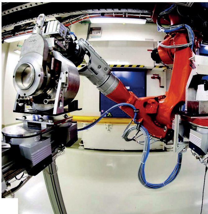
The robot manipulator for handling radioactive materials at the CERN-MEDICIS facility. [Credit CERN].
