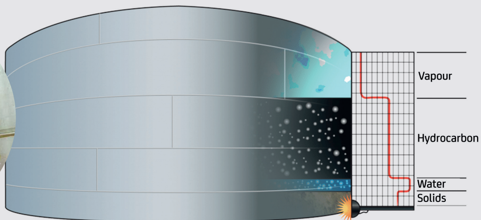
Levels and interfaces in feedstocks in storage tanks can be evaluated using a neutron gauge. [Credit Scantech Nuscan].
