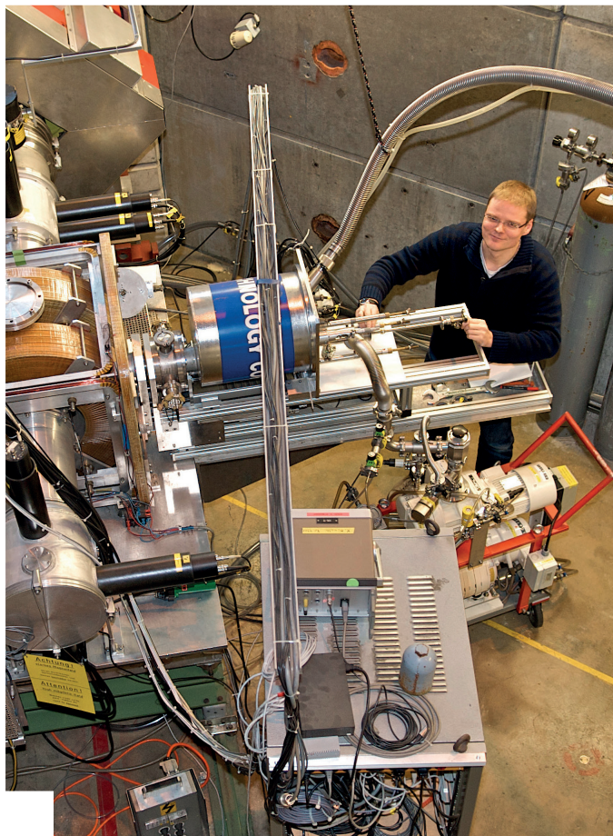
The muon source at the Paul Scherrer Institut in Switzerland used in experiments to study advanced materials. [Credit Paul Scherrer Institut/ Markus Fischer].
