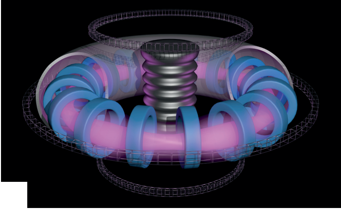
The tokamak (left) and the stellarator employ slightly different approaches to confine a fusion plasma magnetically.
