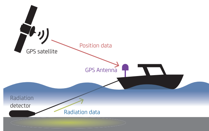
A sketch of the data-acquisition system for sediment transport and pollutant-tracing studies in coastal areas.
