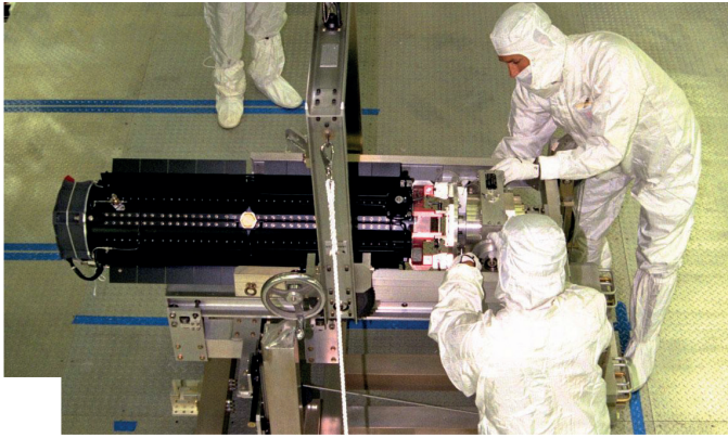
The Cassini-Huygens mission to Saturn relied on a nuclear battery (RTG) for energy, seen here being checked before installation on the spacecraft [Credit NASA].
