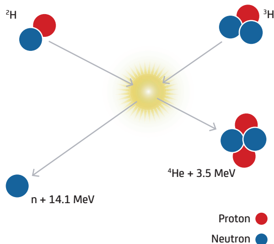
The fusion of deuterium and tritium to helium-4.
