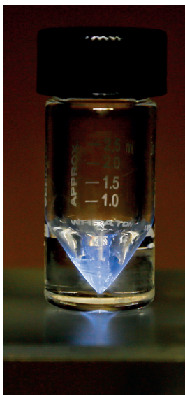
■ A capsule of actinium-225. [Credit ORNL].
