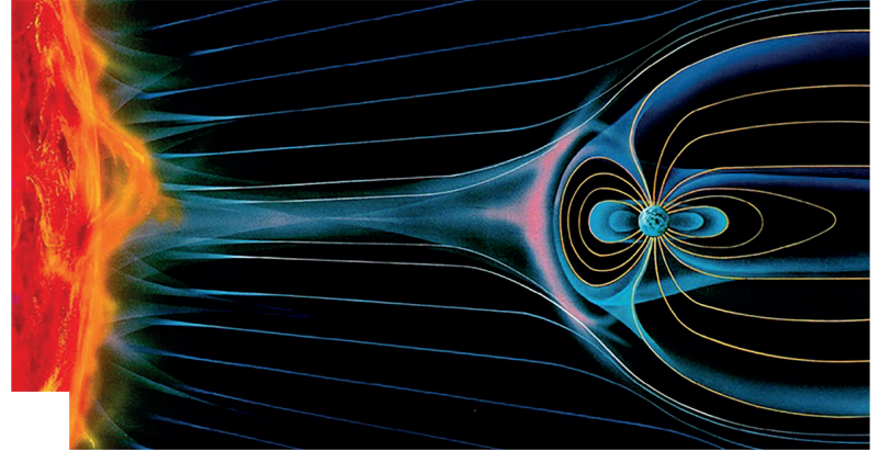
An illustration of the electromagnetic interaction between the solar wind and the Earth's magnetosphere. [Credit ESO/K. Endo].
