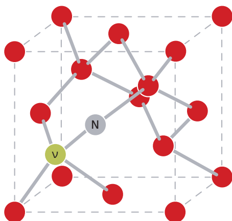
A nitrogen–vacancy qubit in a diamond crystal lattice.
