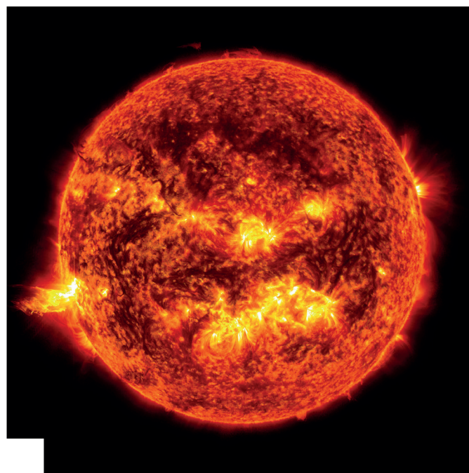
Variations in solar activity such as solar flares have huge effects on weather and climate, which scientists are trying to understand more fully.
