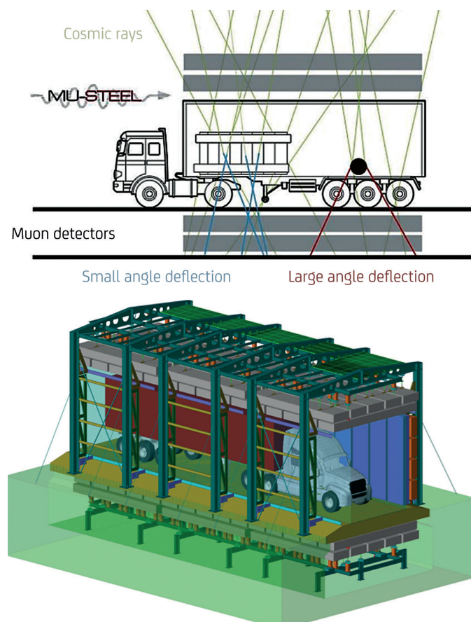
A muon scanner to detect radioactive materials in scrap metal containers. [Credit The Mu-steel EU project].
