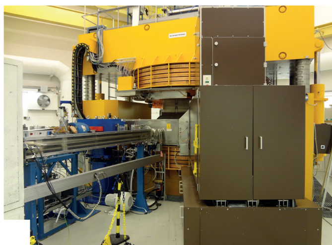
The cyclotron at RADEF in Finland, which is used to test the radiation hardness of electronics to be used in space.
