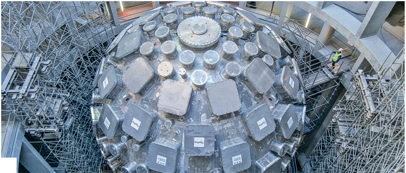
The heart of the Laser Mégajoule ICF facility, seen here during construction. [Credit University of Bordeaux].
