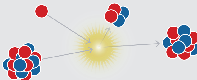
Nuclear studies often involve colliding subatomic particles at high energies to trigger a reaction, and then detecting and measuring the energies of the products.
