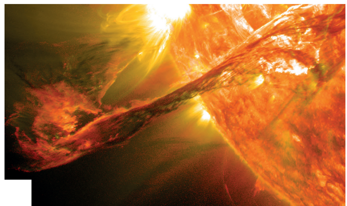
The start of a massive coronal mass ejection in 2012. [Credit NASA/GFSC].
