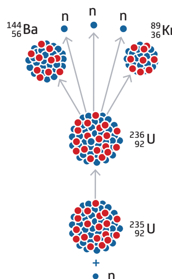
Uranium fission to produce lighter nuclei and neutrons.
