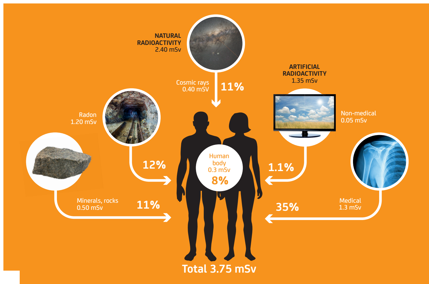
Sources of radiation contributing to an adult average annual dose in Europe (mSv).
