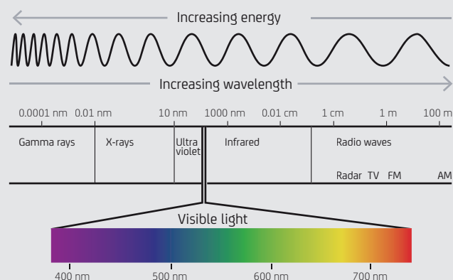
■ The electromagnetic spectrum.
