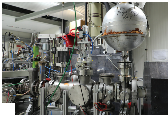
The LUNA laboratory in Italy is dedicated to experiments that explore the nuclear fusion cycles in stars like the Sun. [Credit: The LUNA collaboration].
