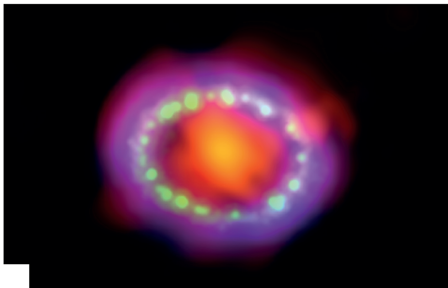
This is a combined multi-wavelength image of the ring of gas and the shockwave generated by the supernova SN1987A that leads to the spreading out of elements in space from which the next generation of stars and planets are made. [Credit X-ray: NASA/CXC/SAO/PSU/D. Burrows et al.; optical: NASA/STScI; millimetre: NRAO/AUI/NSF].
