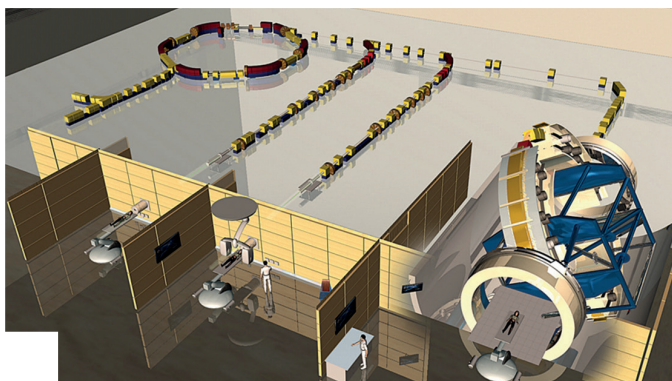
The accelerator setup at HIT in Heidelberg, Germany, where cancer patients can be treated with carbon ions via a massive gantry (at the right) built by GSI engineers. [Credit HIT].
