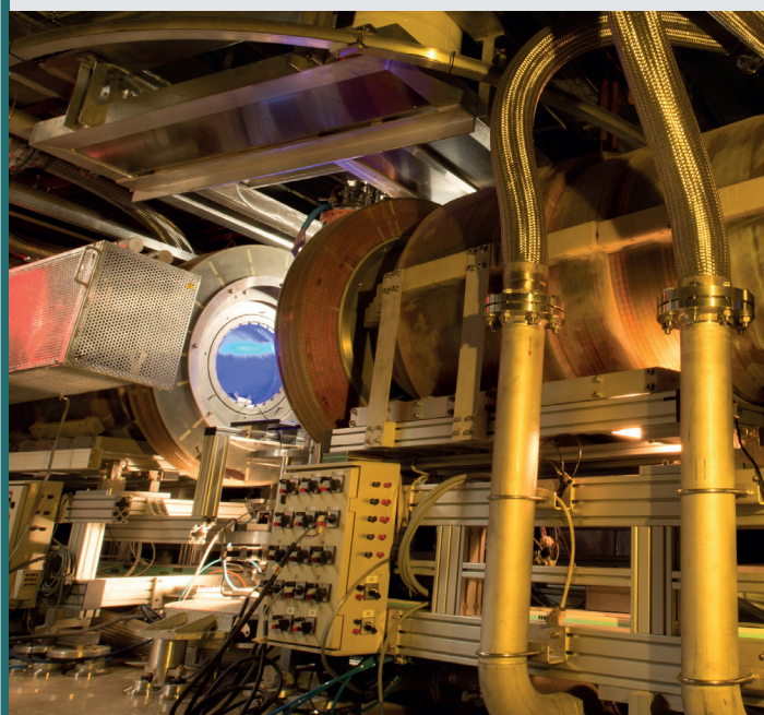
One of the instruments (IN15) at the international ILL facility that utilises an intense neutron beam supplied from its nuclear reactor, and which is tailored for specific experiments in materials science. [Credit Institut Laue–Langevin].
