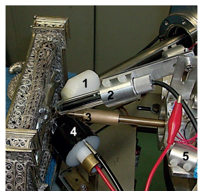
■ Left: The pax of the Vidigueira treasure; right: The pax being analysed with a proton beam. 1: X-ray detector; 2: camera; 3: beam exit nozzle; 4: particle detector; 5: lasers [Credit The Centre for Nuclear Sciences and Technologies, Instituto Superior Técnico, Portugal].
