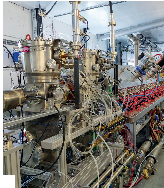
Myrrha's proton injector system.
