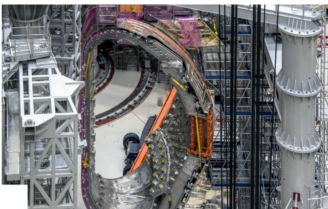
Part of ITER's vacuum vessel with two toroidal field coils and thermal shield segments awaiting assembly. [Credit ITER].
