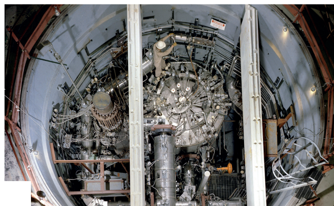
The molten salt reactor using thorium at Oak Ridge National Laboratory in the 1960s. Thorium is again being studied as a fuel for nuclear power.
