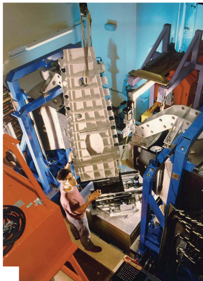
Measuring residual stress in welds in an aircraft wing rib using neutron diffraction which acts as a strain gauge. [Credit STFC ISIS Neutron and Muon Source/ENGIN-X].
