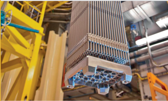
■ A nuclear fuel assembly [Credit Framatome].
