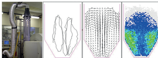
Particle motion in a fluidised bed followed by PEPT. [Credit Positron Imaging Centre, University of Birmingham].
